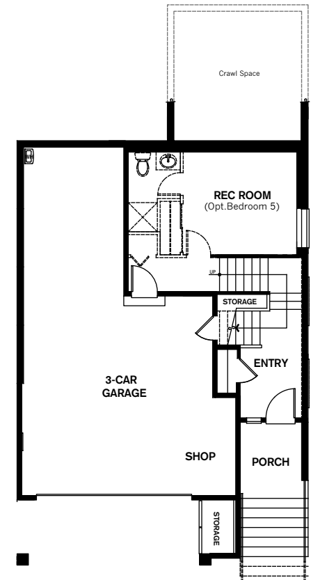
lower FLOORPLAN
