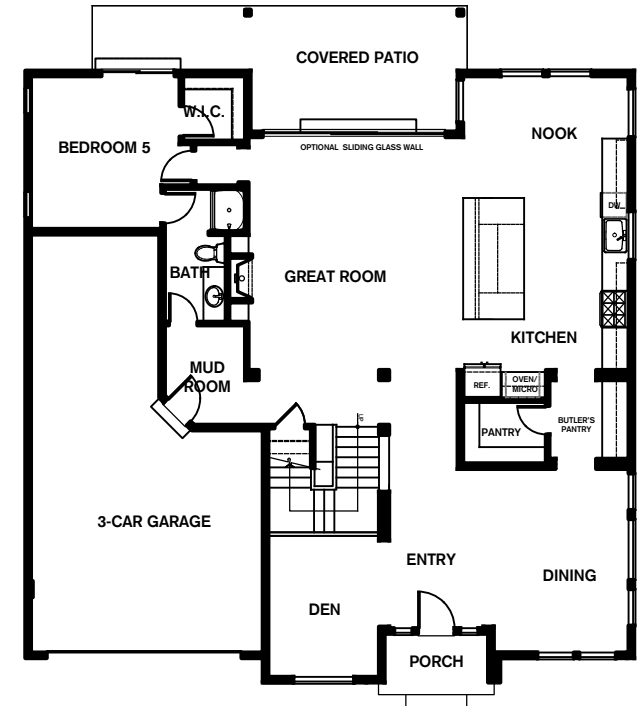
main FLOORPLAN
