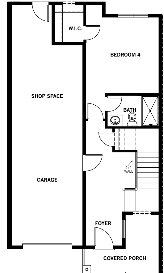
lower FLOORPLAN
