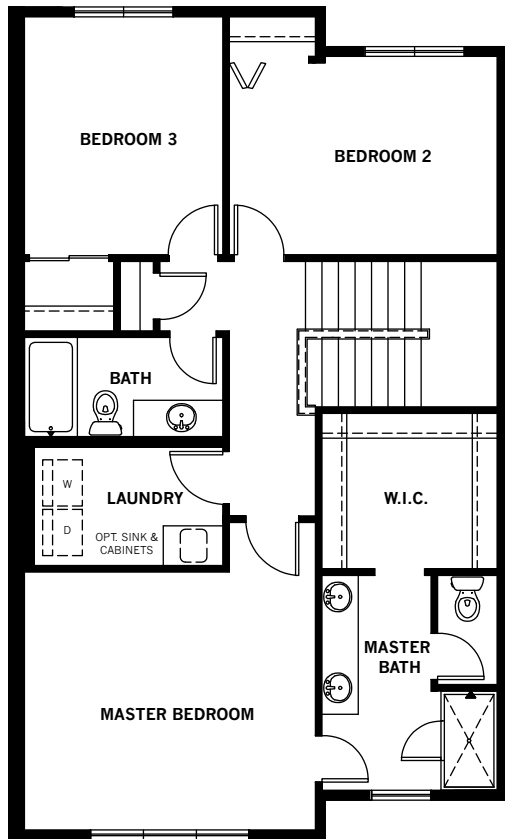
upper FLOORPLAN
