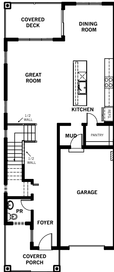
main FLOORPLAN
