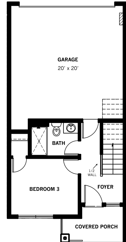
main FLOORPLAN
