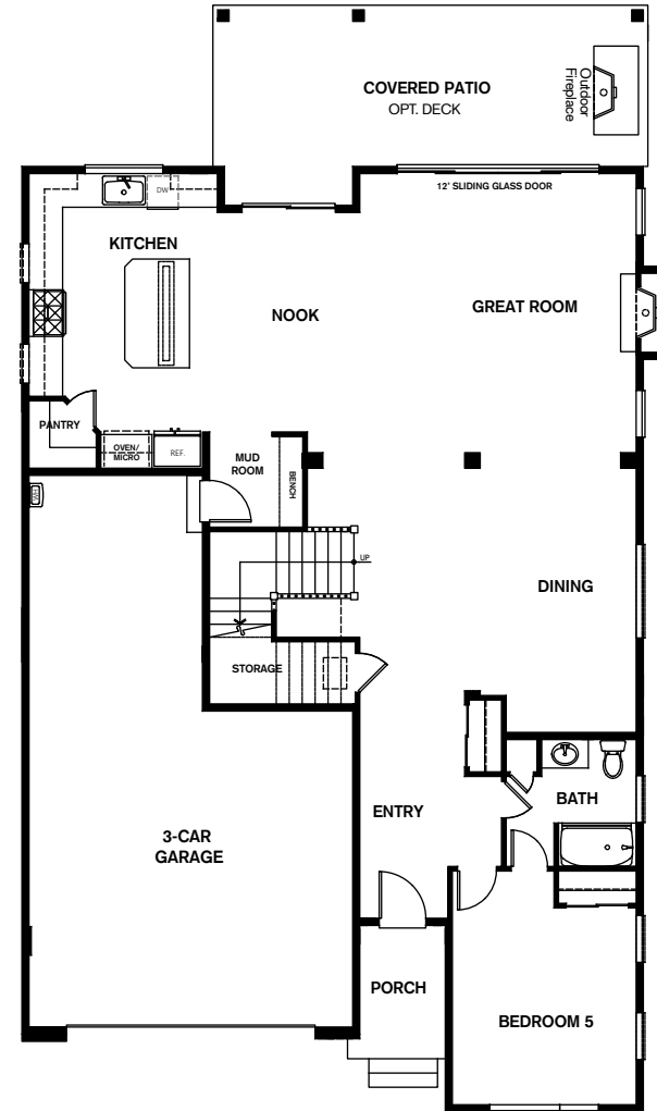
main FLOORPLAN
