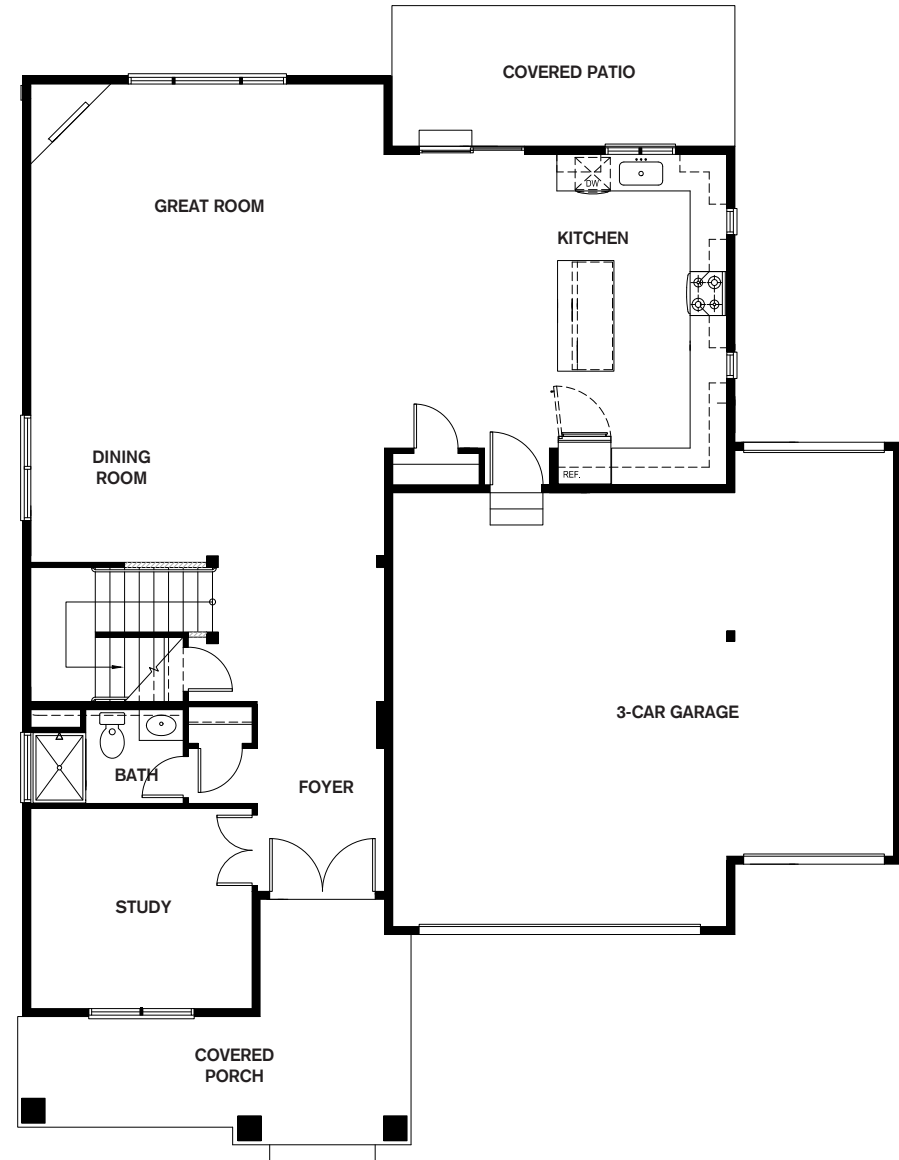
main FLOORPLAN
