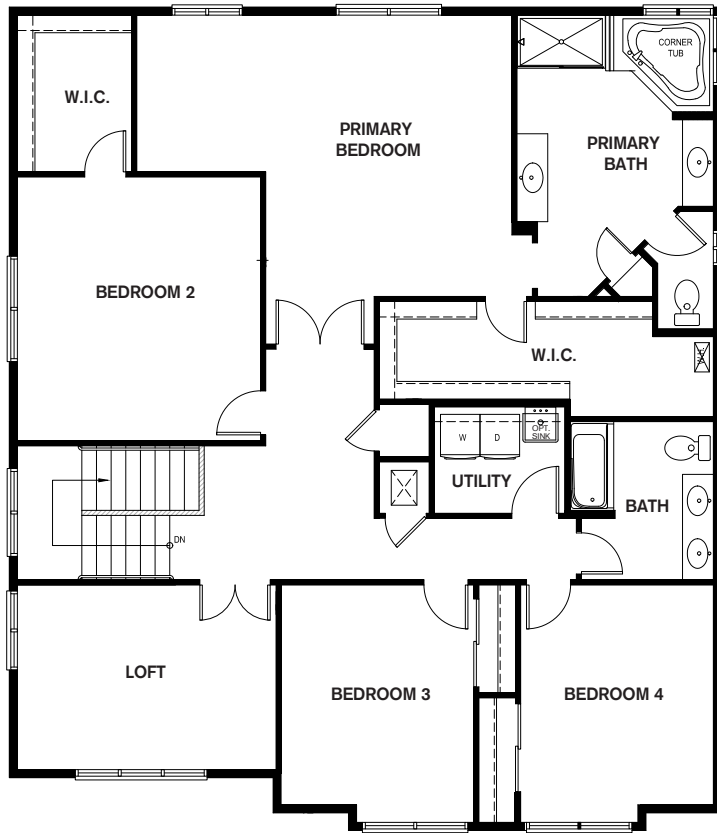
upper FLOORPLAN
