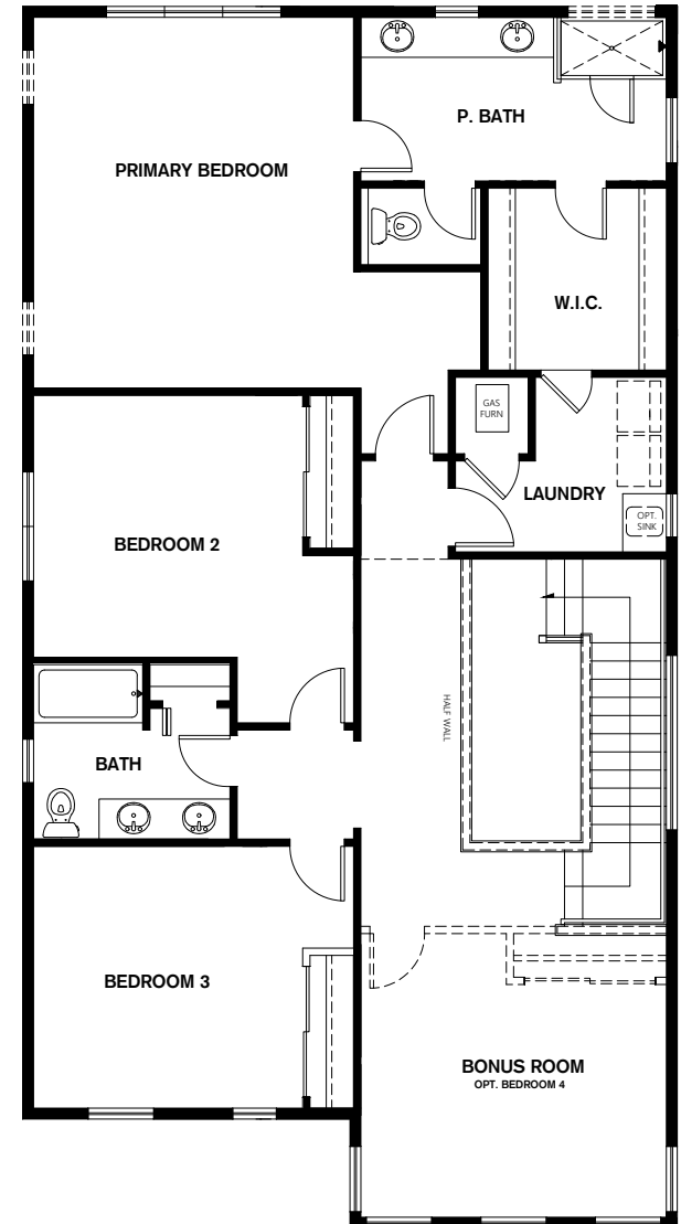
main FLOORPLAN
