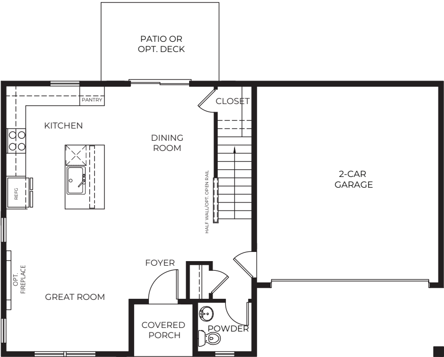
MAIN FLOORPLAN
