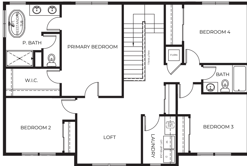
UPPER FLOORPLAN
