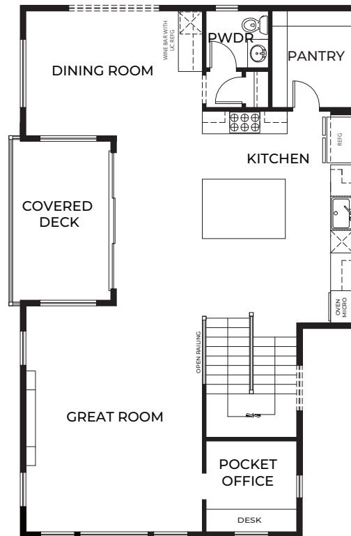
MAIN FLOORPLAN
