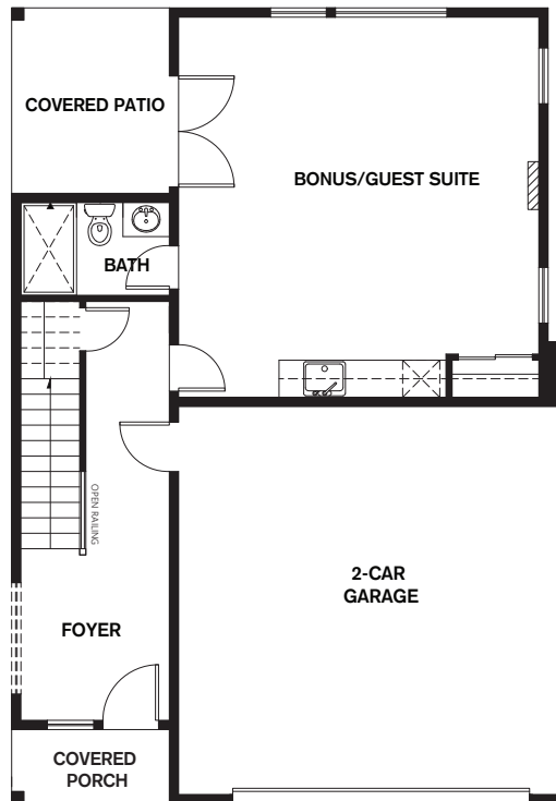
LOWER FLOORPLAN
