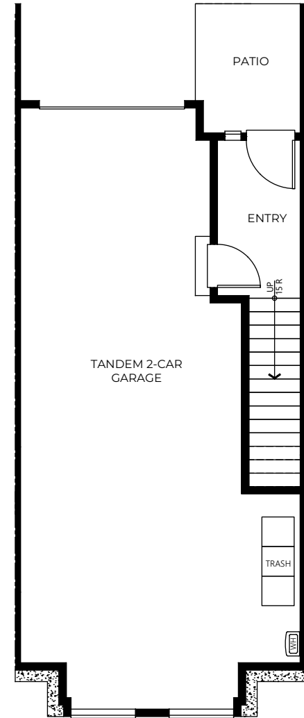
LOWER FLOORPLAN
