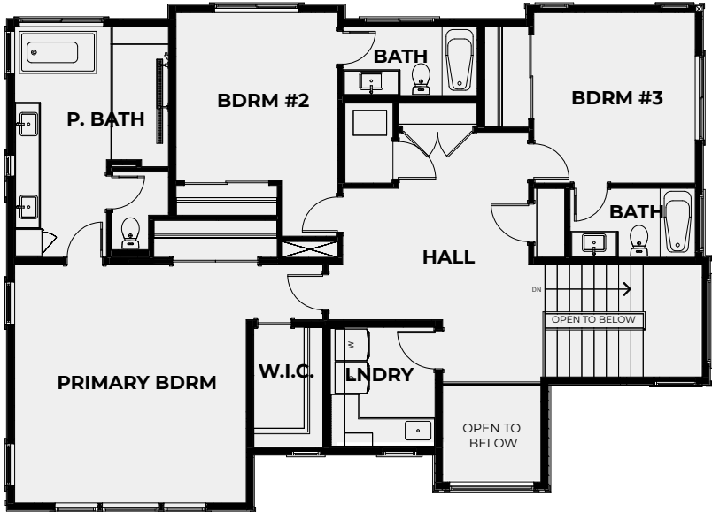
UPPER FLOORPLAN
