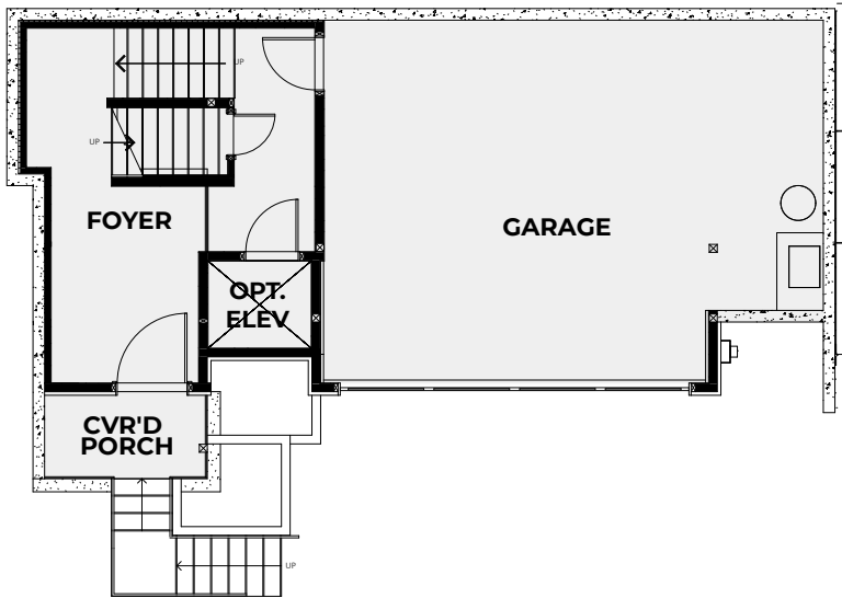
GARAGE FLOORPLAN
