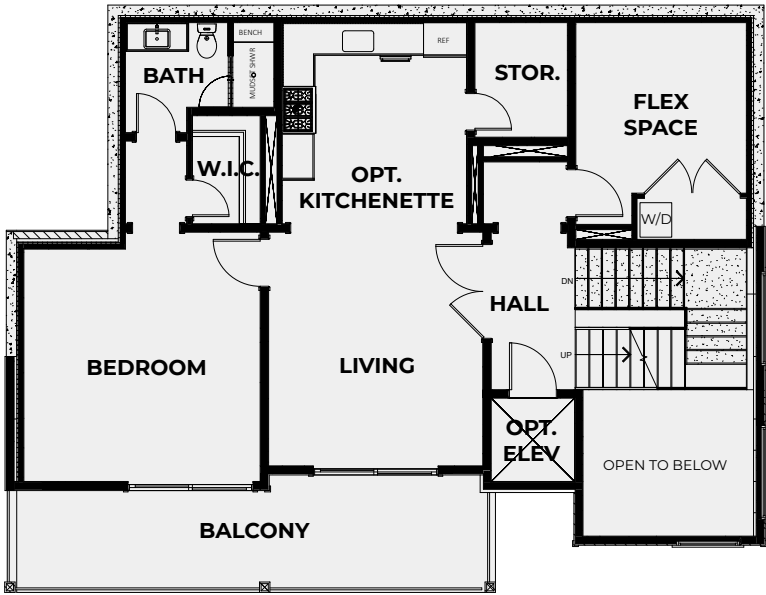
LOWER FLOORPLAN
