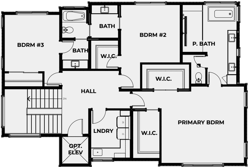
UPPER FLOORPLAN
