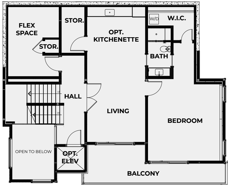
LOWER FLOORPLAN
