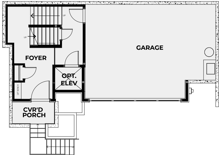
GARAGE FLOORPLAN
