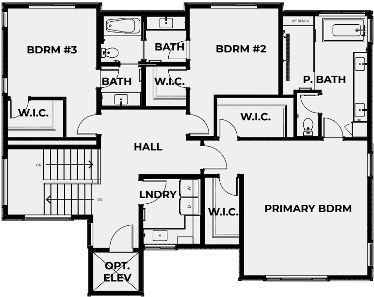
UPPER FLOORPLAN
