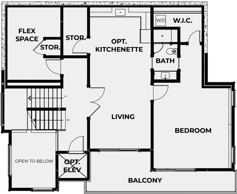
LOWER FLOORPLAN
