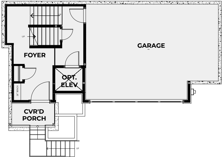
GARAGE FLOORPLAN
