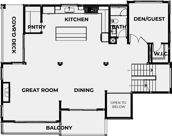
MAIN FLOORPLAN
