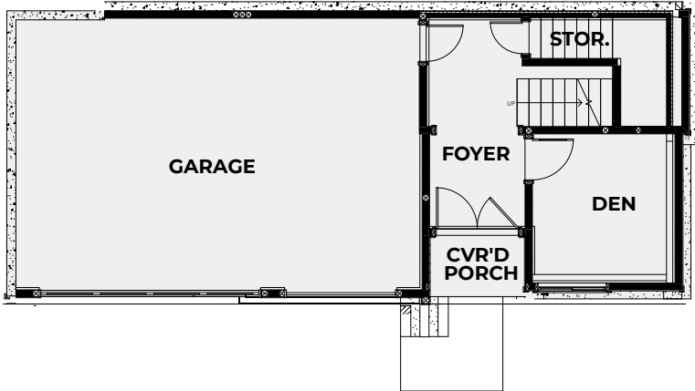
GARAGE FLOORPLAN
