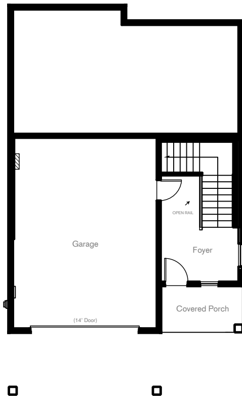
LOWER FLOORPLAN
