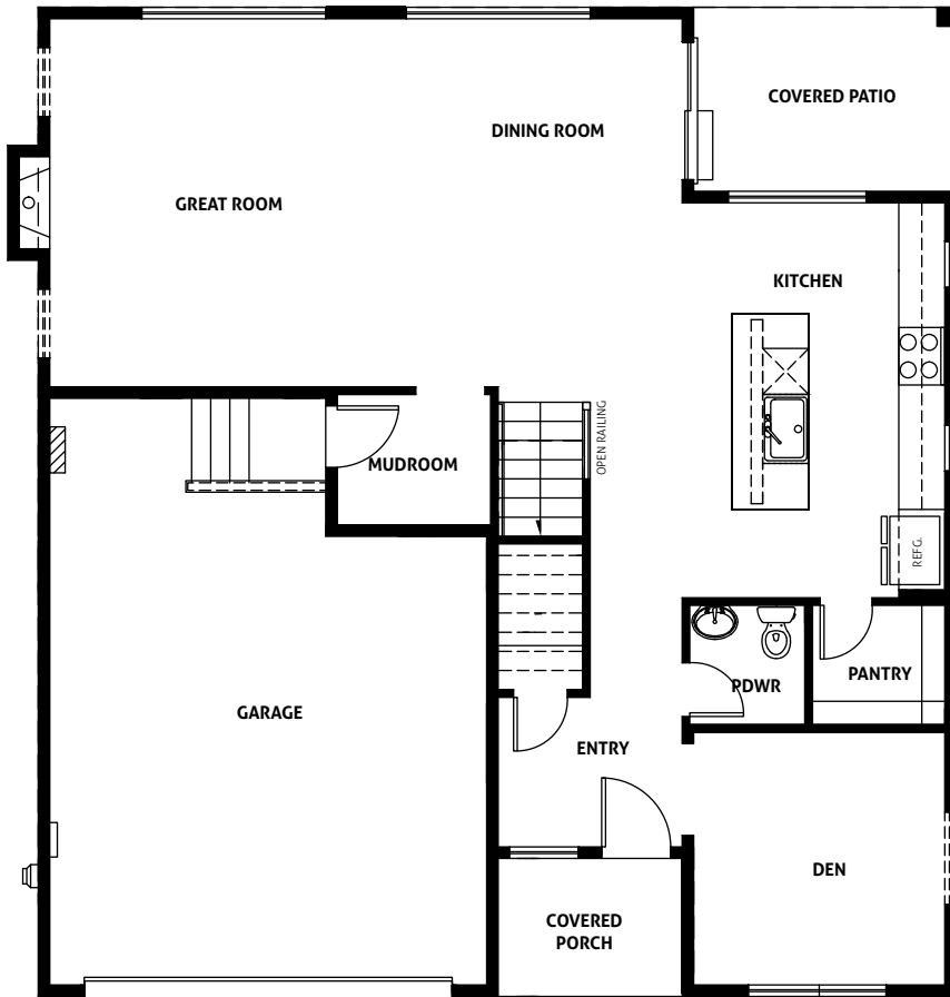
main FLOORPLAN
