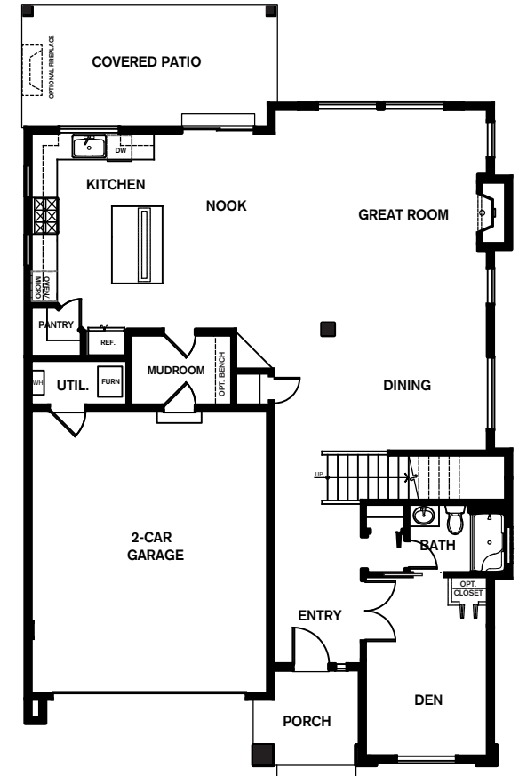
lower FLOORPLAN
