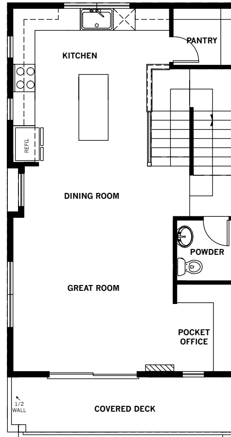
main FLOORPLAN
