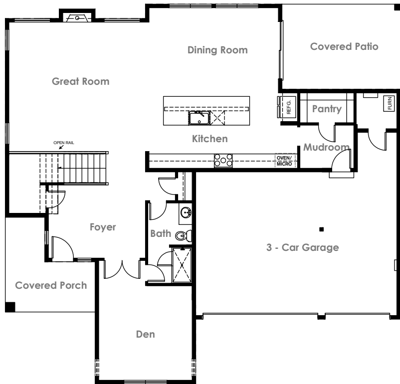
main FLOORPLAN
