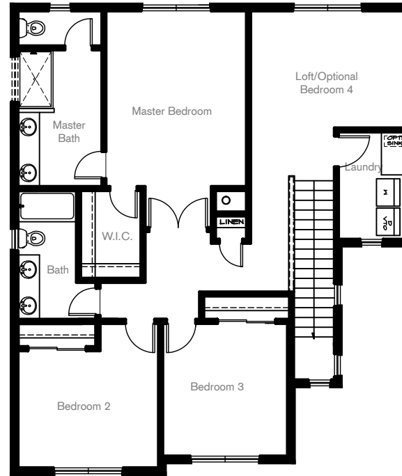
UPPER FLOORPLAN
