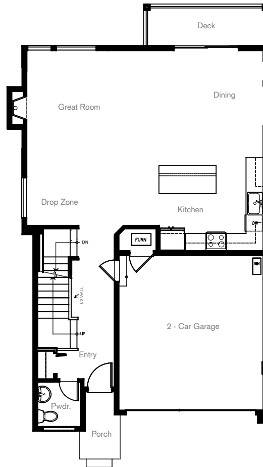
MAIN FLOORPLAN
