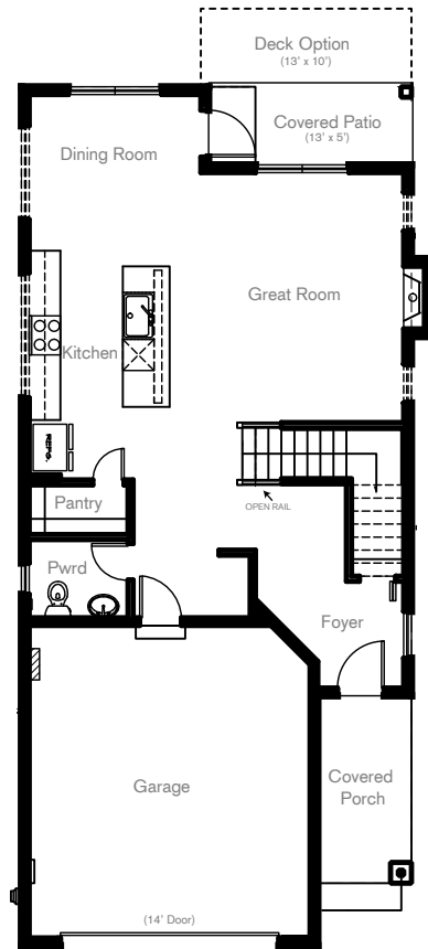
MAIN FLOORPLAN
